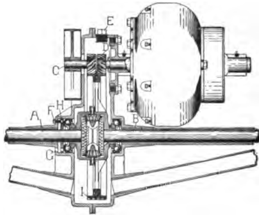
FIG. 437.—Diagram of Single Motor Attached to Rear Axle Through Single Reducing Gears. A is the left-hand section of the divided rear axle; B, the right-hand section of the rear axle; C, the brake drum; D, the spiral pinion on the motor shaft driving the worm gear, I, on the differential; H, ball race on the axle bearing.
